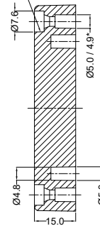
SECTION C-C
