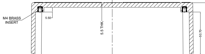
SECTION B-B
