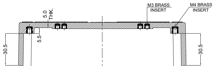
SECTION C-C
